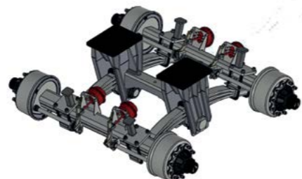
Bogie
