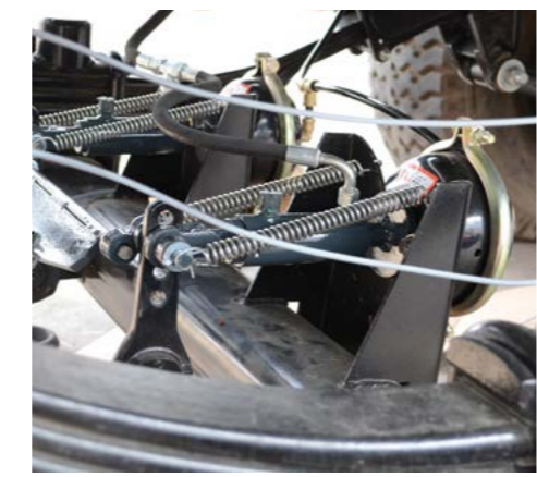
Combined braking system
